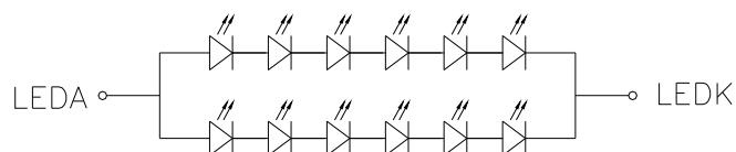
LED Backlight: 2x6 LED
